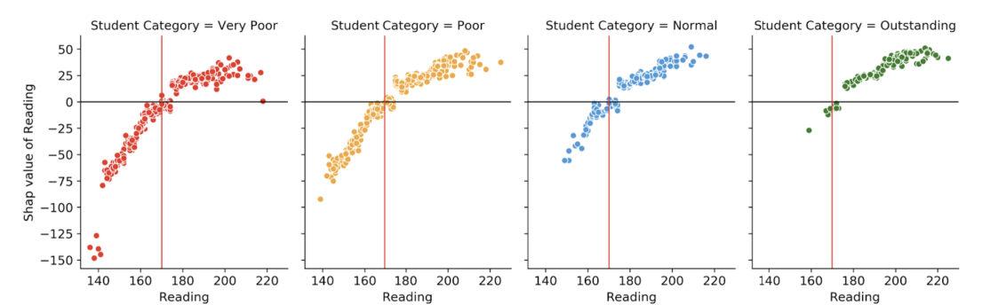
Figure 7 Scatter plot between reading score and SHAP value of reading feature for each student category
