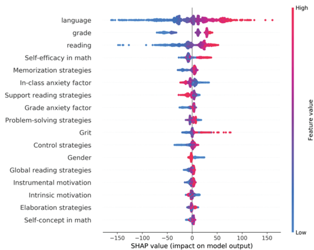
Figure 3 SHAP summary plot of predictive factors by decreasing importance
