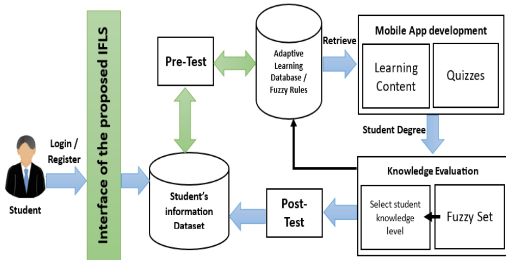
Figure 3. Architecture for the proposed FILS
